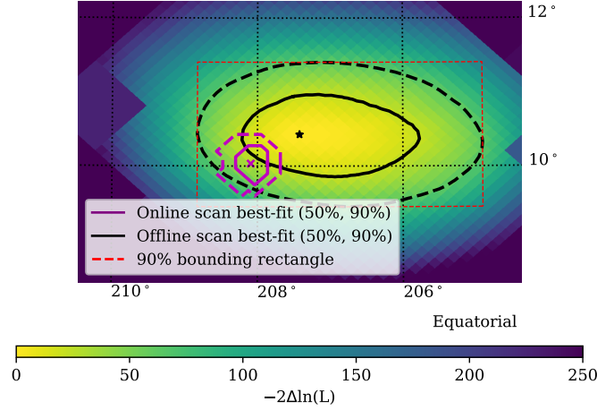
Figure 1: Example of a log-likelihood map of a neutrino alert reconstructed with the full-sky maximum likelihood reconstruction algorithm in right ascension and declination. The black star is the best-fit position from the likelihood scan. The solid and dashed black curves represent the 50% and 90% confidence level respectively, derived from the likelihood scan. The red dashed rectangle determines the errors quoted in the GCN Circulars and is defined as the minimum rectangle that would encapsulate the uncertainty contours. Lastly, the purple solid and dashed curves are the 50% and 90% confidence level contours calculated with the initial, less refined reconstruction method and sent out in the first GCN Notice.
