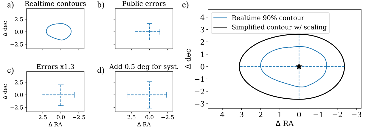
Figure 4: Example of the simplification and scaling that is applied to the realtime contours in Plavin et al. (2020), which is also done in the cross check presented here. From the original contours in Panel a), only the minimum rectangle is published, which is translated to uncertainty in the coordinates (Panel b). Those errors are multiplied by 1.3 (Panel c) and an extra parameter is added to account for systematic uncertainties, leading to a minimum p -value at an added 0.5 degrees (Panel d). The error bars are joined by elliptical segments to obtain the simplified contours corresponding to the best-fit position from the reconstruction, represented by the black star (Panel e).
