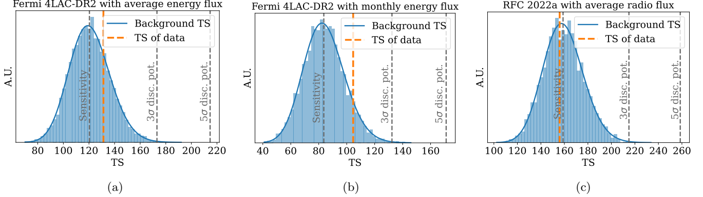
Figure 3: The blue histogram shows the distribution of the TS values for N = 5000 background maps, fitted to a gamma distribution (blue curve). The orange dotted line represents the observed TS of the data, while the grey lines represent the TS_{\text{data}} needed to reject the background hypothesis at the 3\sigma or 5\sigma level. Panel a) For the Fermi 4LAC-DR2 catalog with the average energy flux weights, TS_{\text{data}} = 131.3 , while TS = 120.4 for the median background maps, leading to a p -value of 0.248. Panel b) For the Fermi 4LAC-DR2 catalog with the monthly energy flux weights, TS_{\text{data}} = 104.6 , median background maps has TS = 83.6 and the p -value is 0.08. Panel c) For the RFC 2022a catalog, TS_{\text{data}} = 155.8 , TS = 158.9 for the median background maps and the p -value is 0.57.
