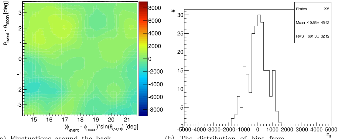
(a) Fluctuations around the background model of an off-source region, defined in relation to the position of the Moon. The color axis is the best-fit number of total signal events given the response at that point.
