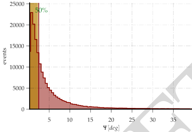
Figure 4: The \Psi distribution integrated over all simulated muon angles and energies. The line indicates the median of the distribution.
